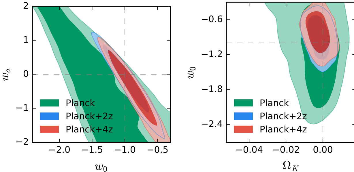
Figure 6. Left panel: 2D marginalized contours for 68% and 95% confidence level for w_0 and w_a ( w_0w_a CDM model assumed) from Planck-only (green), Planck+CMASS (1 bin)+LOWZ (1 bin) (blue), and Planck+CMASS (2 bins)+LOWZ (2 bins) (red); right panel: 2D marginalized contours for 68% and 95% confidence level for \Omega_k and w_0 ( ow_0w_a CDM model assumed). One can see that w_0 and w_a are consistent with -1 and 0 respectively which correspond to the \Lambda CDM.
