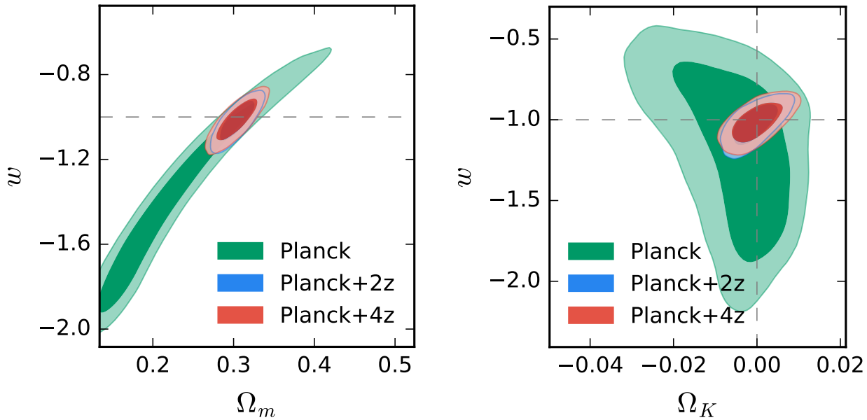
Figure 5. Left panel: 2D marginalized contours for 68% and 95% confidence level for \Omega_m and w ( w CDM model assumed) from Planck-only (green), Planck+CMASS (1 bin)+LOWZ (1 bin) (blue), and Planck+CMASS (2 bins)+LOWZ (2 bins) (red); right panel: 2D marginalized contours for 68% and 95% confidence level for \Omega_k and w ( ow CDM model assumed). One can see that \Omega_k is consistent with 0 and w is consistent with -1 which corresponds to the \Lambda CDM.
