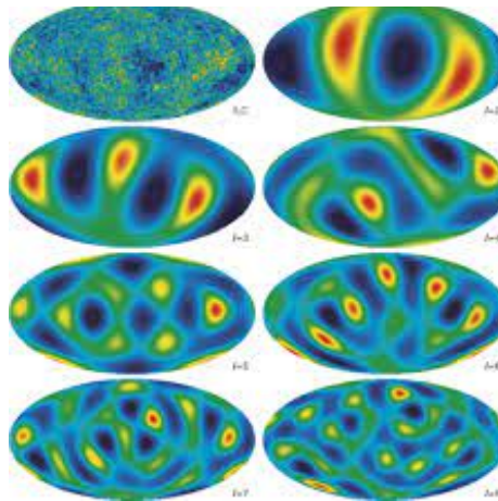
Figure 1: CMB temperature.
