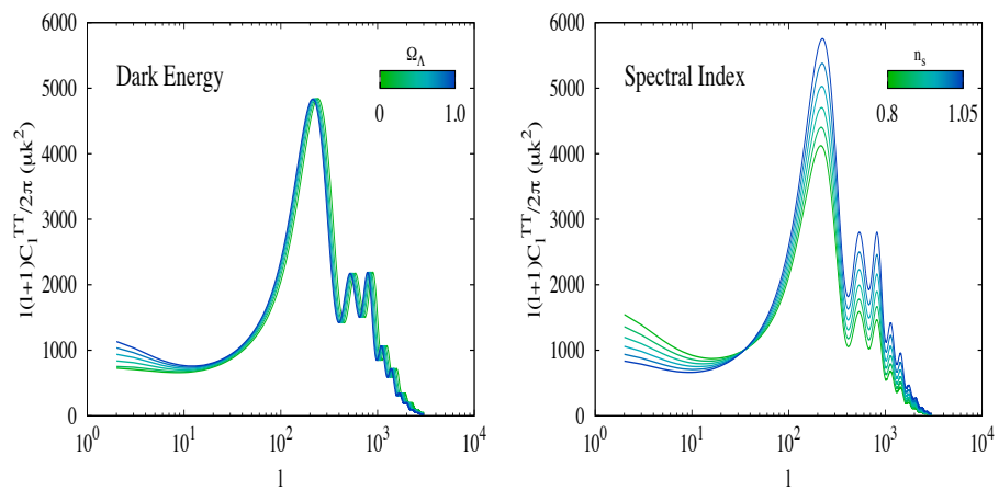
Figure 1: Likelihood grid.
